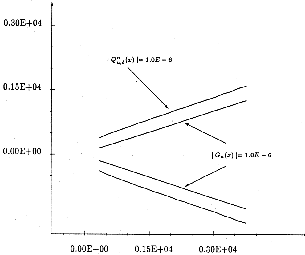
Figure 4: Functions Q_{u,\delta}^n , G_{u,\delta} , with u = 168 , n = 311 , \delta = 13.82 \approx -\log(1.0E-6)
