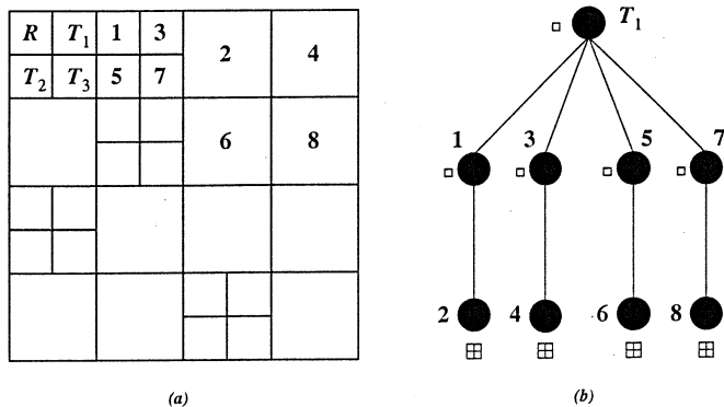
Figure 3: (a) Sample segmentation in a 3-level wavelet packet decomposition, and (b) the parent-offspring dependencies for compatible zerotree originating from T_1 .
