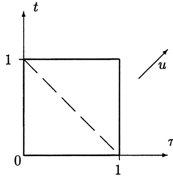
Figure 4.1: The split of integration range that yields (4.19)
