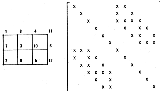
Figure 3: Alternate Diagonal Ordering and Its Type 1 Matrix
