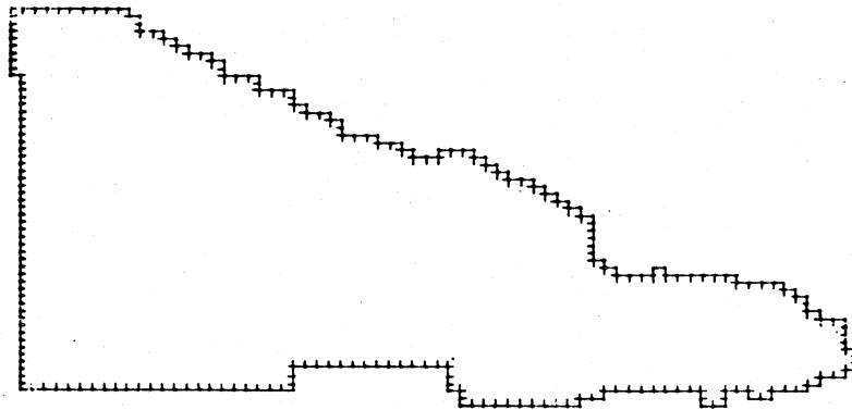
Figure 6: Simulation Problem 3, 55x72, 2,347 Equations
