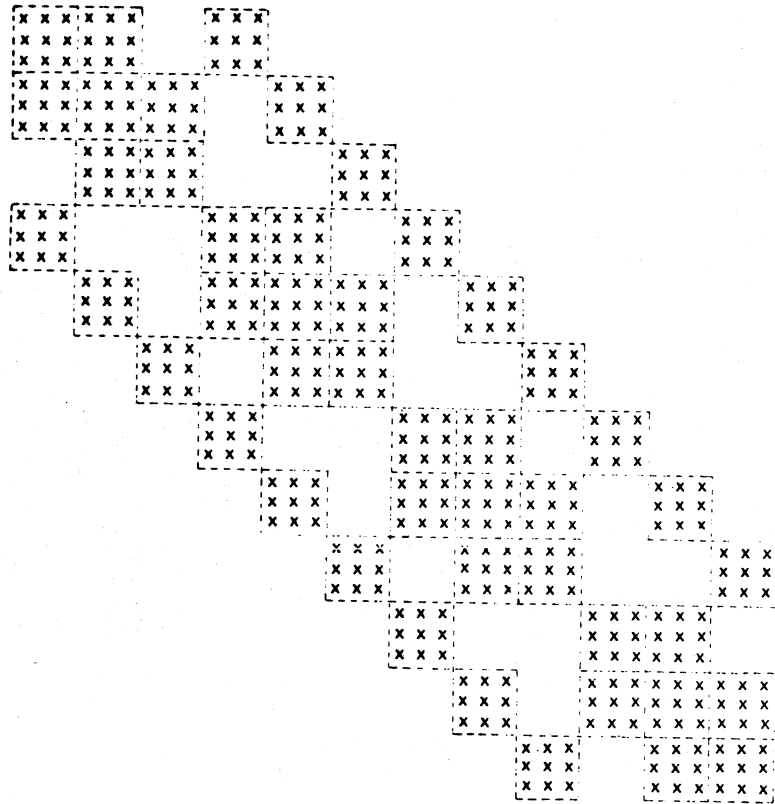
Figure 2: Type 2 (Block) Matrix from a 3x4 Grid
