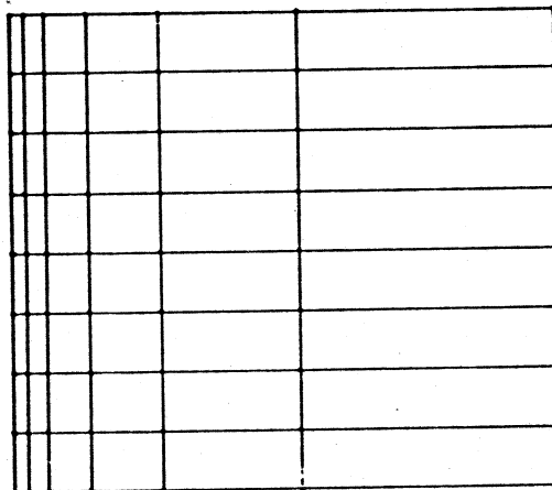
Figure 7: Simulation Problem 4, 7x9, 189 Equations
