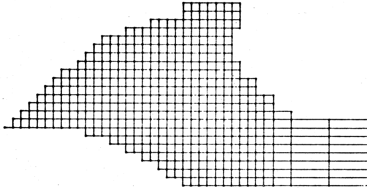
Figure 5: Simulation Problem 2, 23x37, 507 Equations
