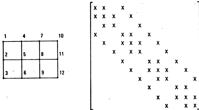
Figure 1: Type 1 Matrix from a 3x4 Grid.
