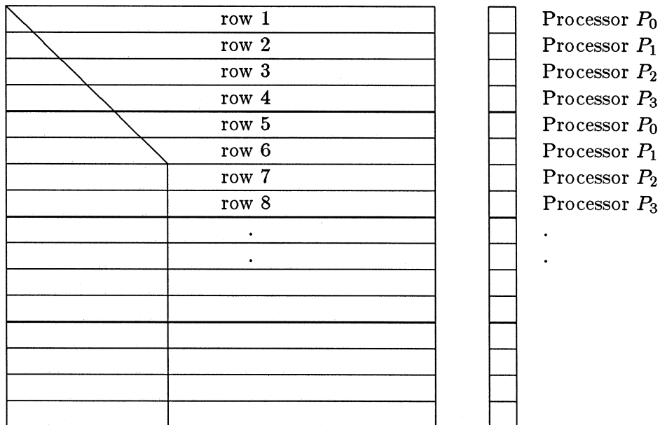
Figure 3: Gaussian Elimination with Interleaved Rows for k = 4 .
