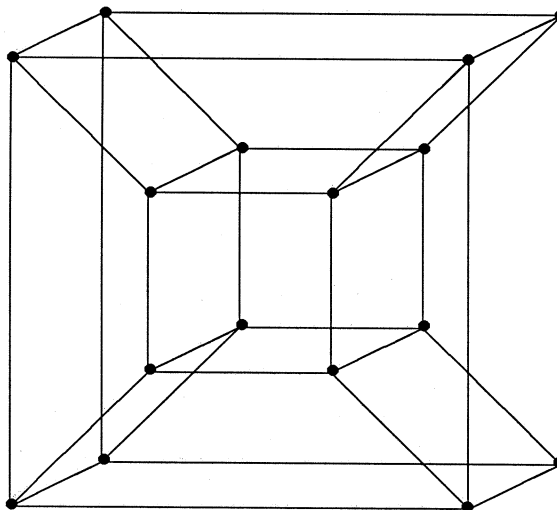
Figure 1: A Hypercube of Dimension 4.
